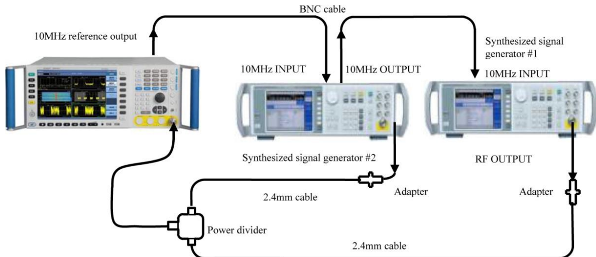
Fig. 8.5 Schematic diagram of frequency span accuracy test
