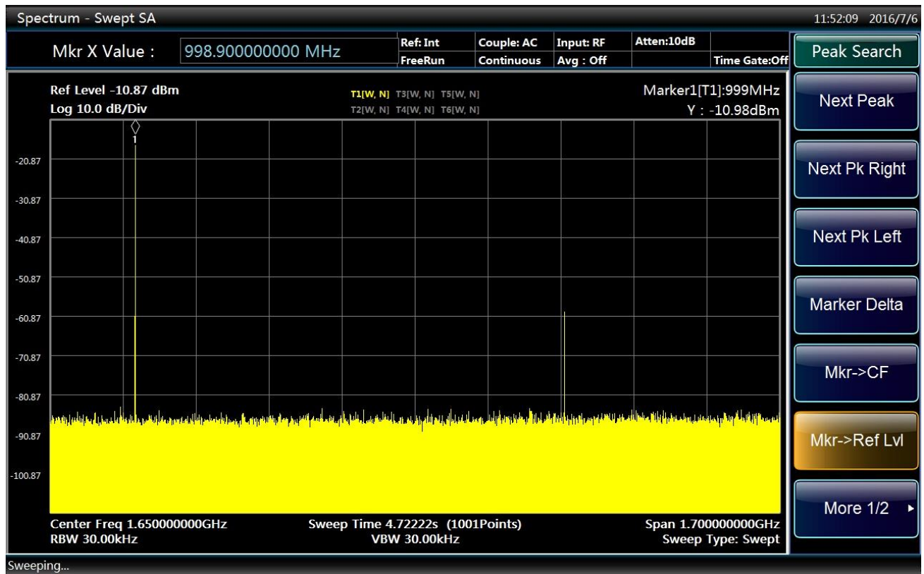
Fig. 4.18 Display interface of signal peak at reference level
