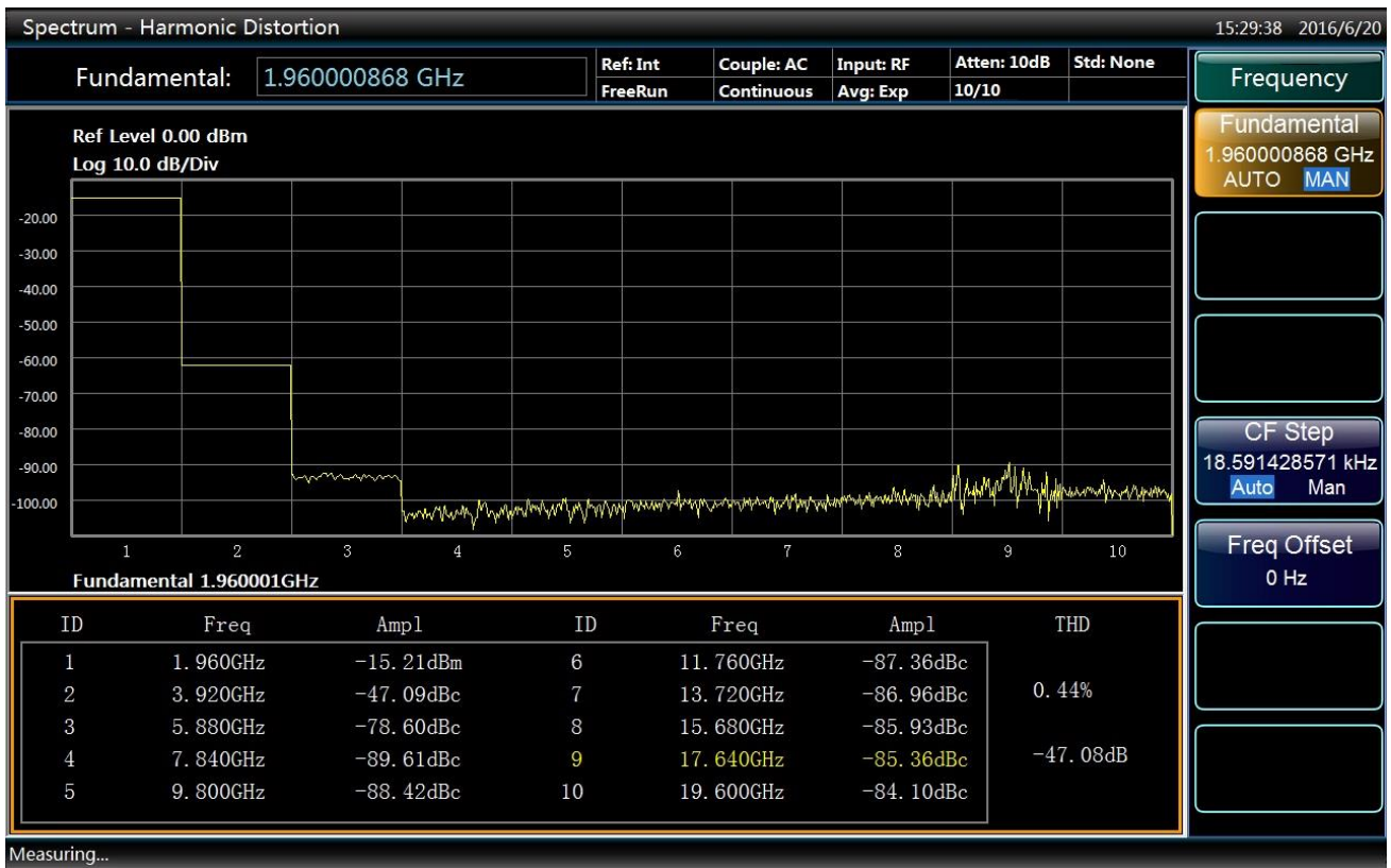
Fig. 4.77 Results of Harmonic Distortion Measurements
