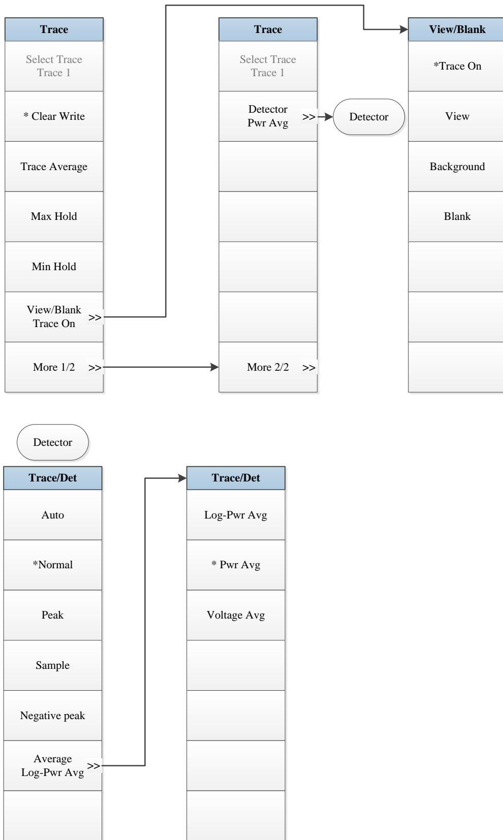
Fig. 5.3-7 Trace Menu
