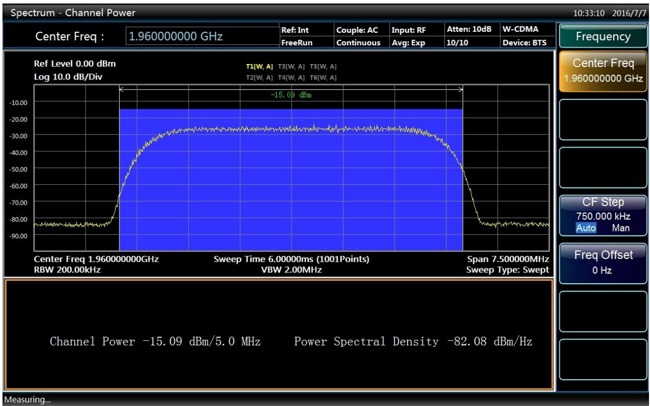
Fig 4.62 Results of channel power measurement
